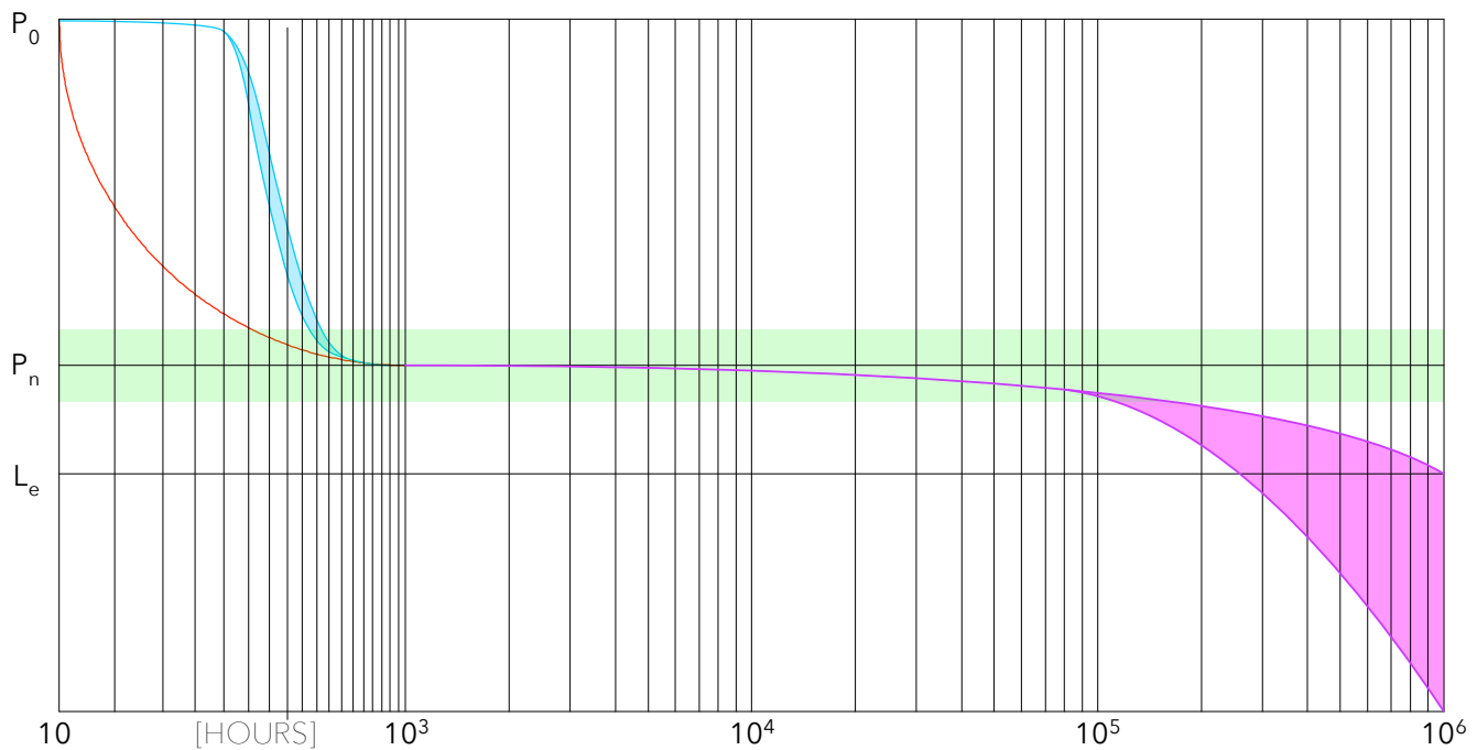
DIRTY WEEKEND-6 SUPERFLY LOUDSPEAKER SYSTEM FATIGUE PROFILE [2023]
