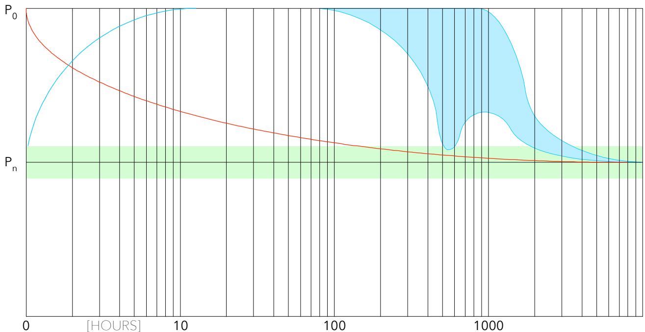
DIRTY WEEKEND-6 SUPREME BURN/BREAK-IN PROFILE [2023]
