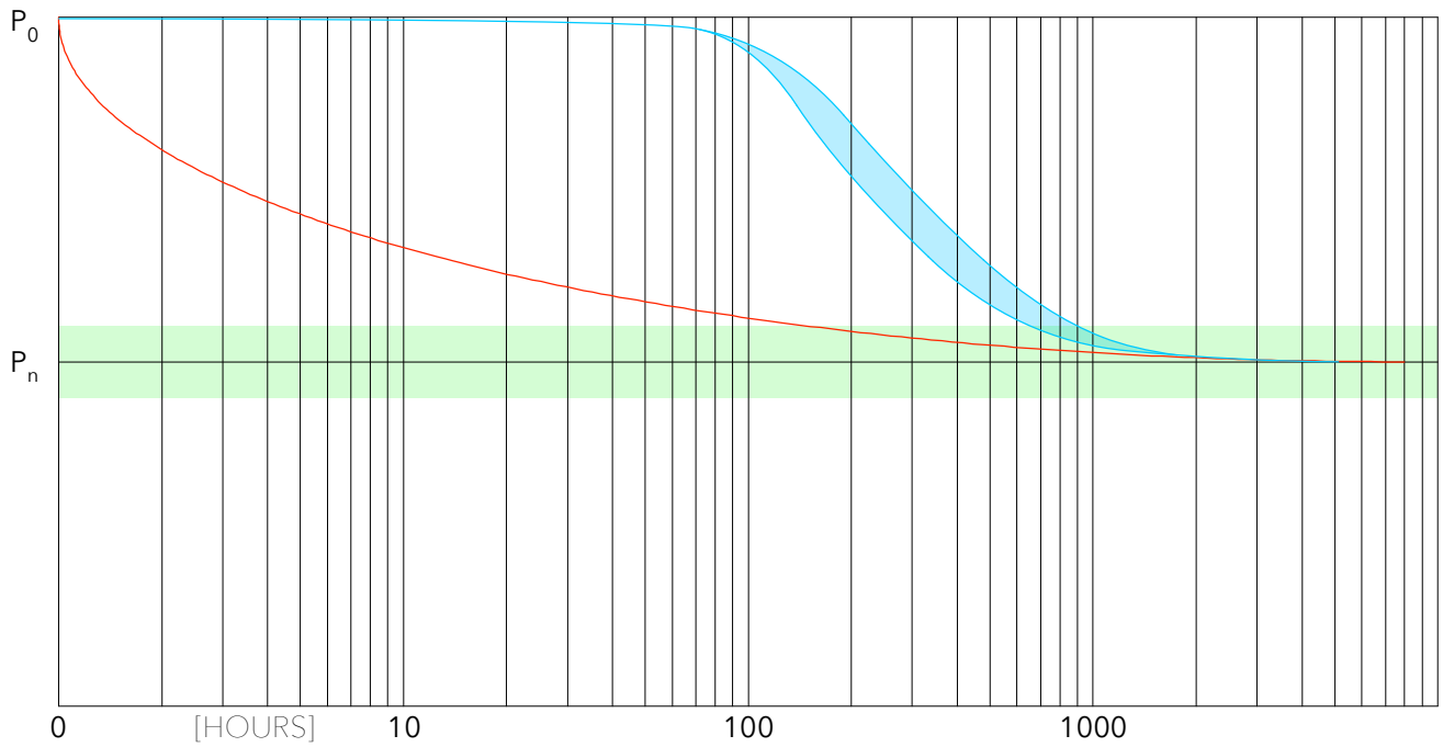
UNION-6 BURN/BREAK-IN PROFILE [2/2023]
